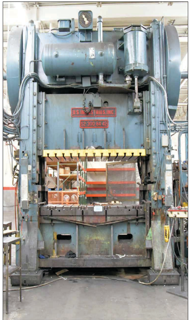
US Industries S2-300-84-42, 300 Ton Capacity Air Clutch Straight Side Press
